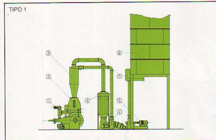
BRICMATIC 1-65/150
